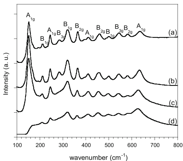
Figure 3 Raman spectra of the (a) B-lactate, (b) B-NaOH, (c) B-HCl, and (d) B-Ti(III)/(IV) brookite samples.
