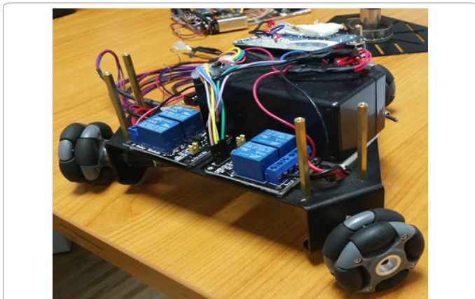
Figure 2: The Robotic Mechanical Base Description, Omni Wheel Chassis Holding DC Motors.
