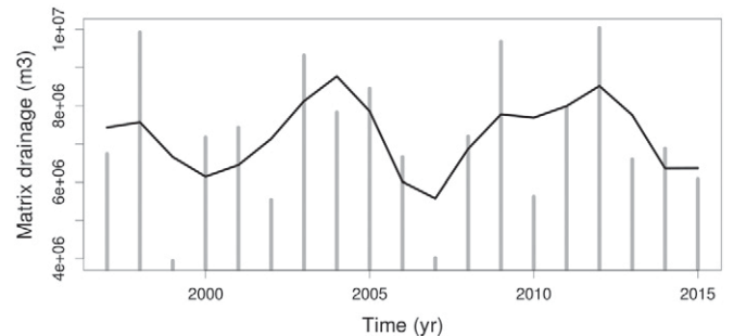
Fig. 8. Annual volume of simulated matrix drainage to conduit network (vertical gray bars) at the Lez site and its low-frequency \sim 6 -yr oscillatory component (solid black line) extracted by wavelet multi-resolution decomposition.
