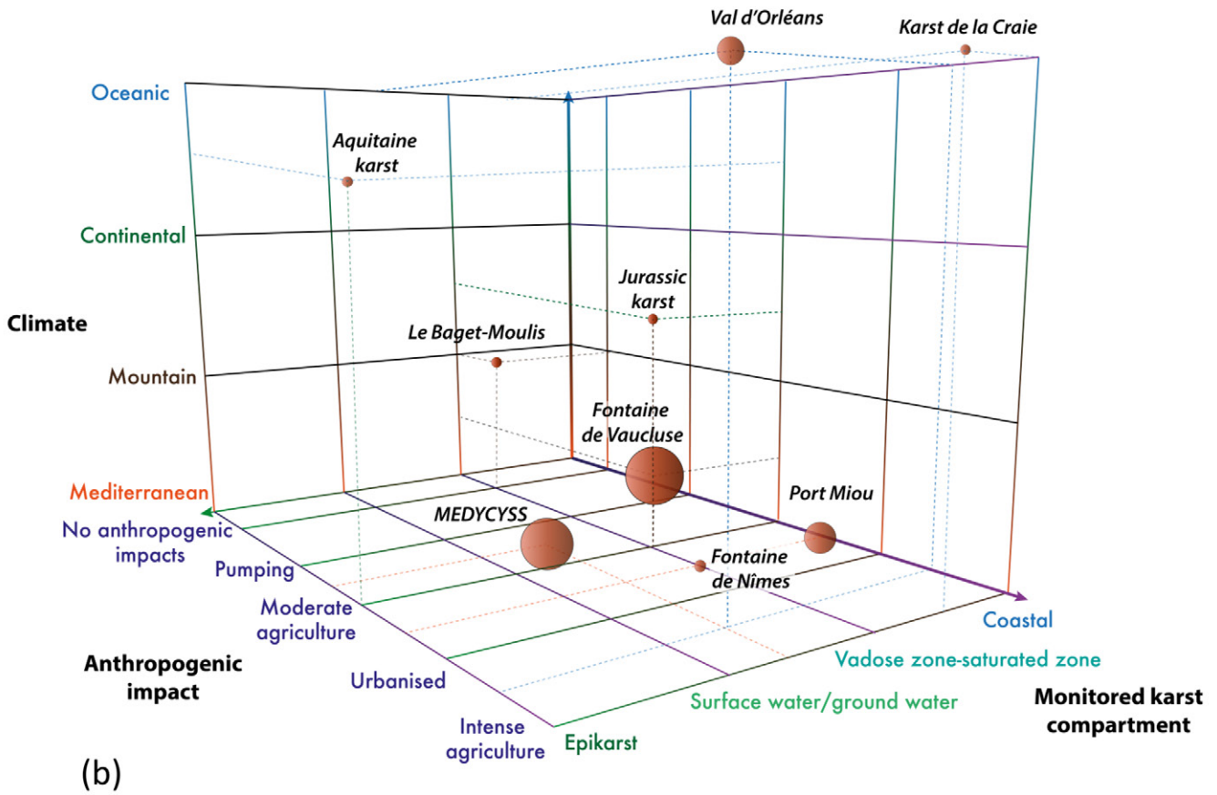
Fig. 1. (a) Location of the observatory sites that compose the French Karst National Observatory Service (SNO KARST), and name of the earth sciences and astronomy observatories (OSUs) and laboratories in charge of their monitoring. (b) Diversity of hydrogeological, hydrological, and hydro-chemical settings of the various observatory sites; circle size is proportional to the catchment area (see Table 1 for more details).
