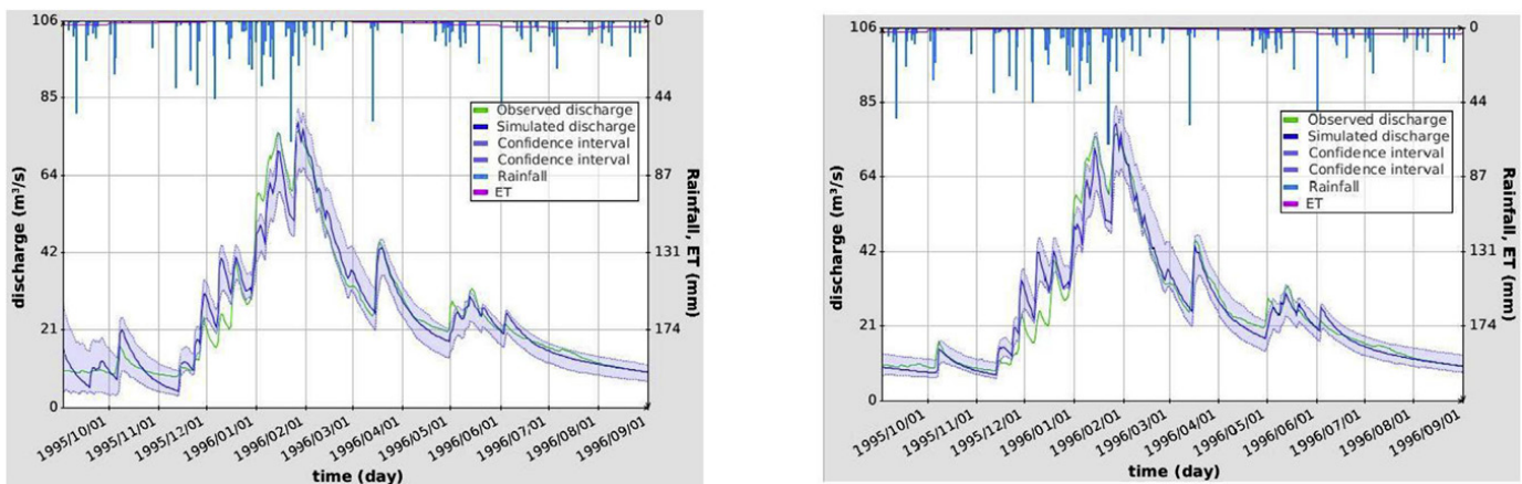
Fig. 4. KarstMod provides a variety of tools for simulation analysis and equifinality assessment. Here, simulation results are provided together with their confidence interval for the behavioral parameter set (Nash Sutcliffe efficiency > 0.9) during the calibration stage: (left) no warmup period, (right) a 1-yr warmup (per Mazzilli et al., 2017). ET stands for evapotranspiration.
