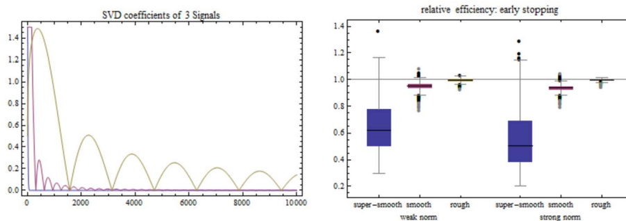
FIG 1. Left: SVD representation of a super-smooth (blue), a smooth (red) and a rough (olive) signal. Right: Relative efficiency for early stopping with m_0 = 0 .
