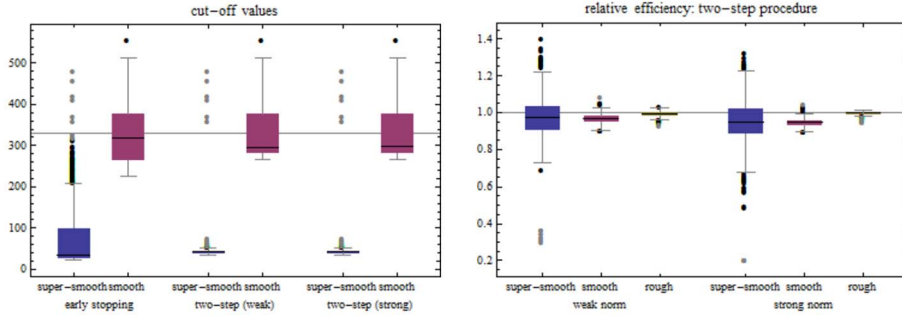
FIG 2. Left: truncation levels for early stopping with m_0 = 0 and the two-step procedures with m_0 = \lfloor q_{0.99}\sqrt{2D} \rfloor + 1 = 329 , AIC in weak and strong norm. Right: Relative efficiencies for the two-step procedure.
