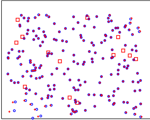
Fig. 2. Topology constructed by the centralized algorithm. The beacons are represented by \square , sensors positions by + , and their estimations by \circ .
