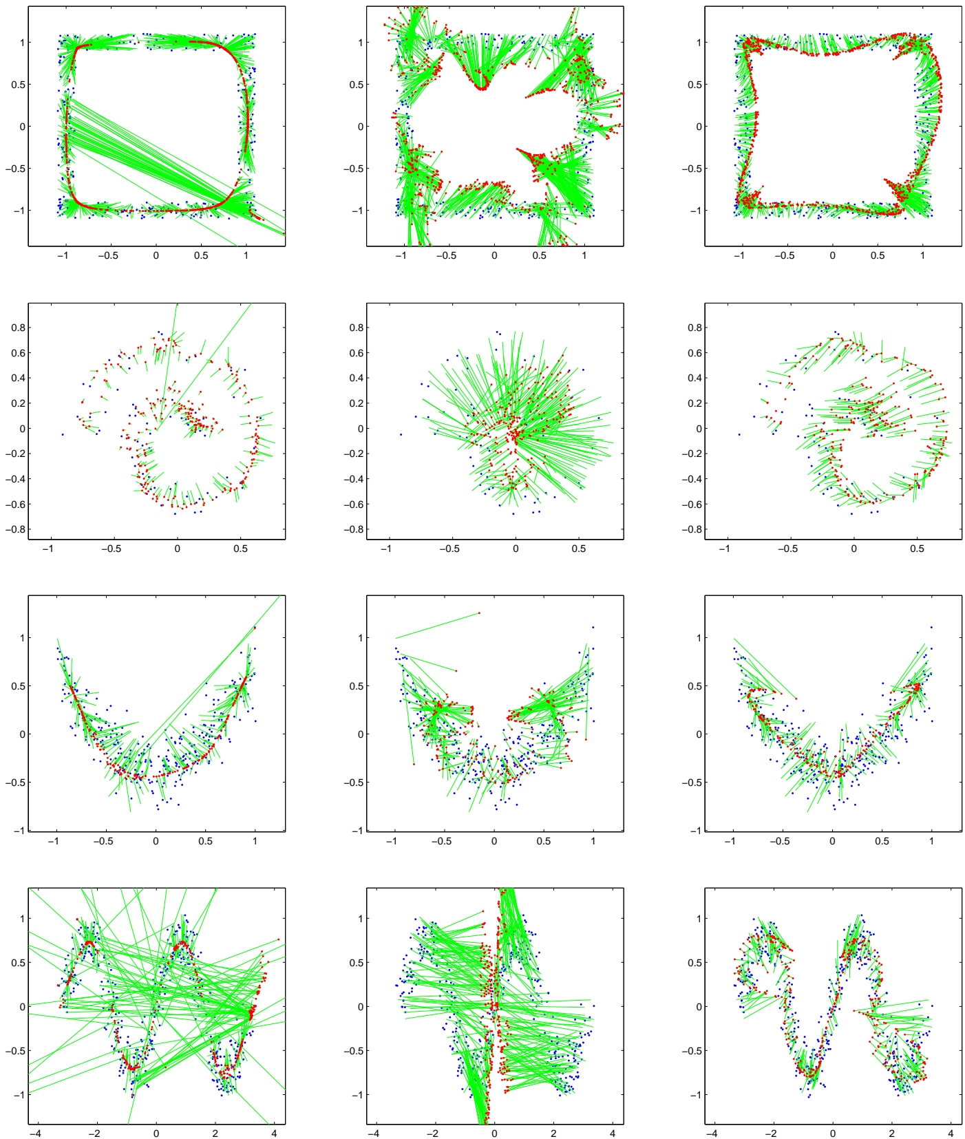
Fig. 1. Results obtained using the iterative (left), the MDS-based (middle), and the proposed (right) algorithm, for the frame (first row), the spiral (second row), the banana (third row), and the sine (fourth row) datasets. Training data are represented by blue dots, estimated pre-images by red dots, and green lines illustrate the distance between these denoised pre-images and the initial noisy data (not shown).
