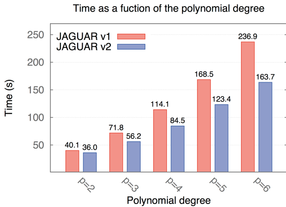
Figure 8: Computational time (in s) as a function of the polynomial degree for both initial and optimized versions of JAGUAR .
