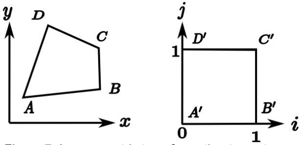
Figure 7: Isoparametric transformation to cast a mesh cell ABCD into the square A'B'C'D'
