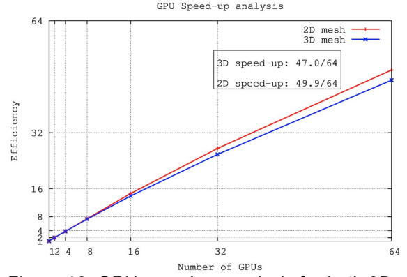
Figure 16: GPU speed-up analysis for both 2D and 3D meshes.
