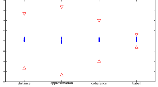
Fig. 1. Illustration of Theorem 10 for the four studied sparsification criteria. The corresponding upper and lower bounds are illustrated with “ \nabla ” and “ \triangle ”, respectively, and the isometry ratio in (23) is evaluated on a set of 200 samples, illustrated with “.”.
