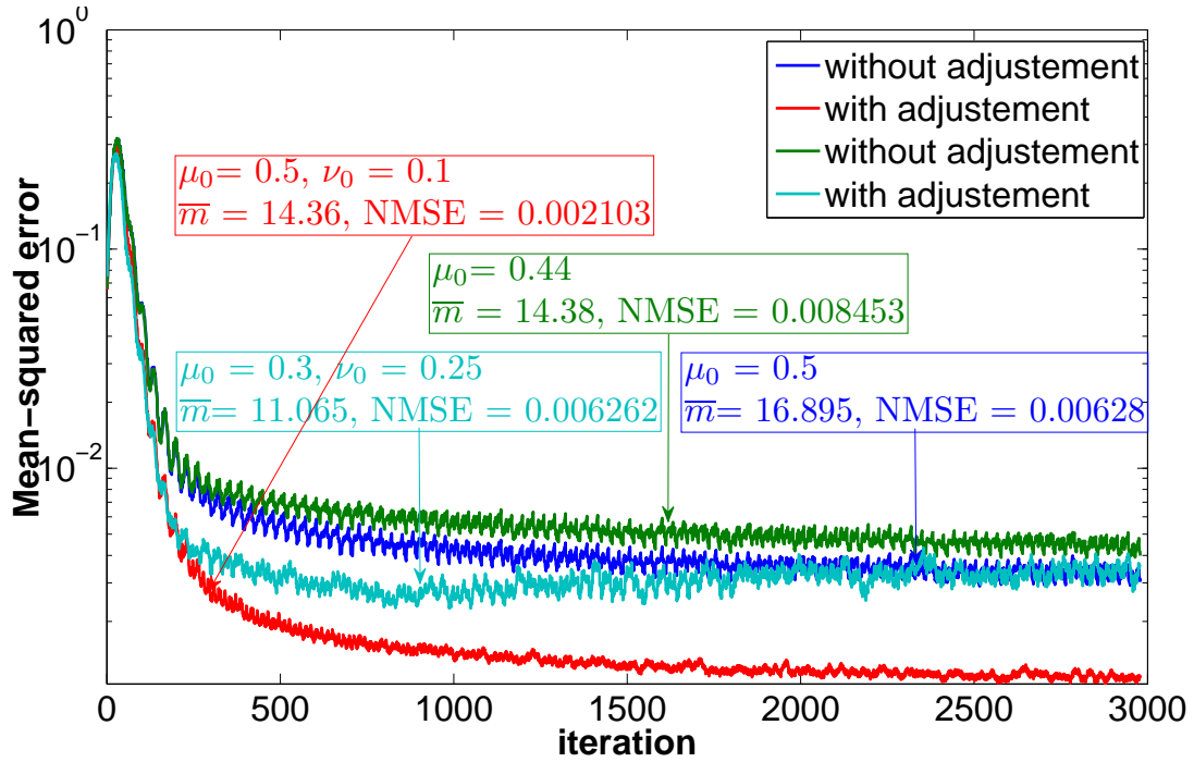
Figure 10. KNLMS: Mean Squared Error with and without adaptation - gaussian kernel
