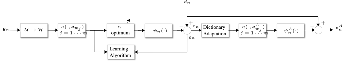
Figure 1. Global adaptation algorithm.
