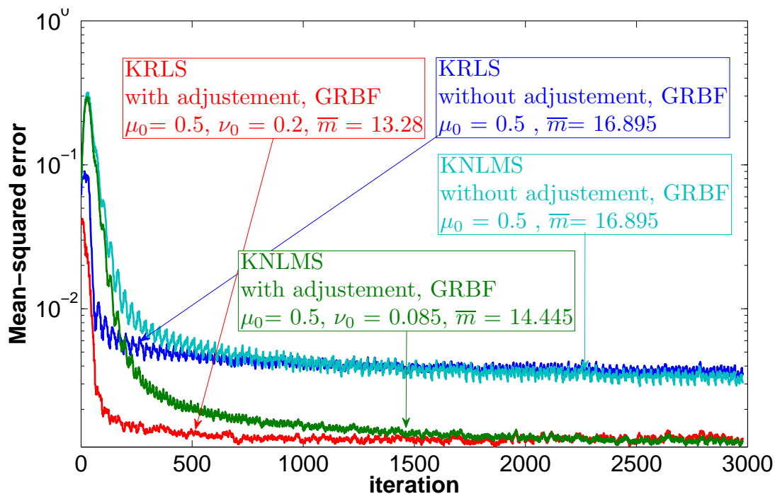
Figure 12. KNLMS versus KRLS - gaussian kernel
