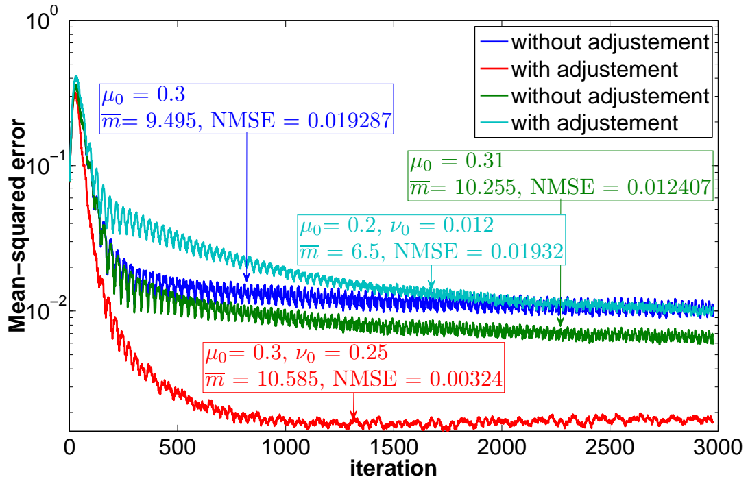
Figure 11. KNLMS: Mean Squared Error with and without adaptation - exponential kernel
