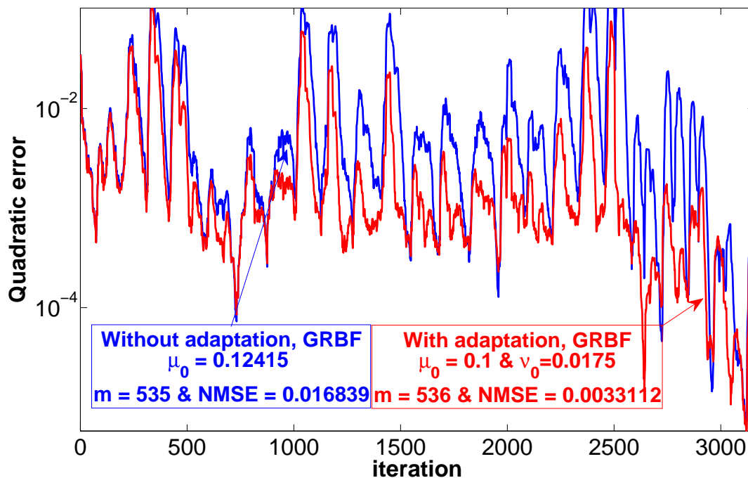
Figure 13. Sunspots prediction using the gaussian kernel
