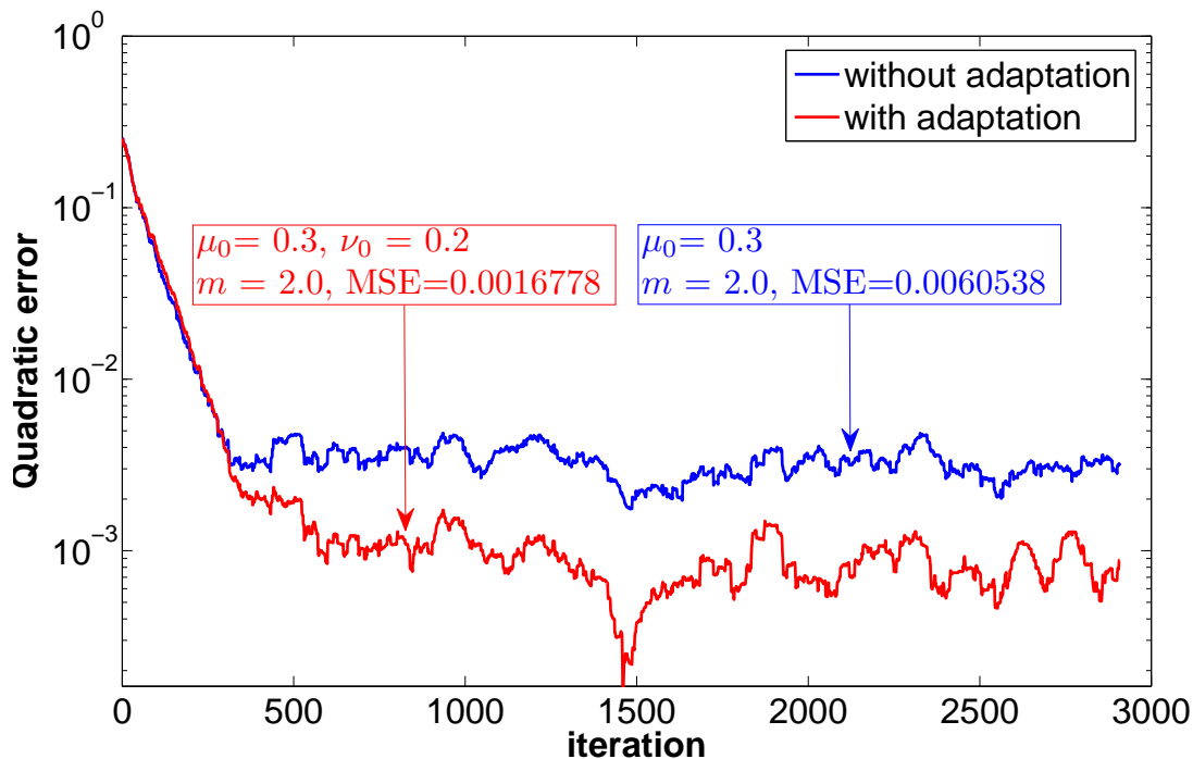
Figure 6. Logistic Map: Quadratic Error - KAPA with gaussian kernel
