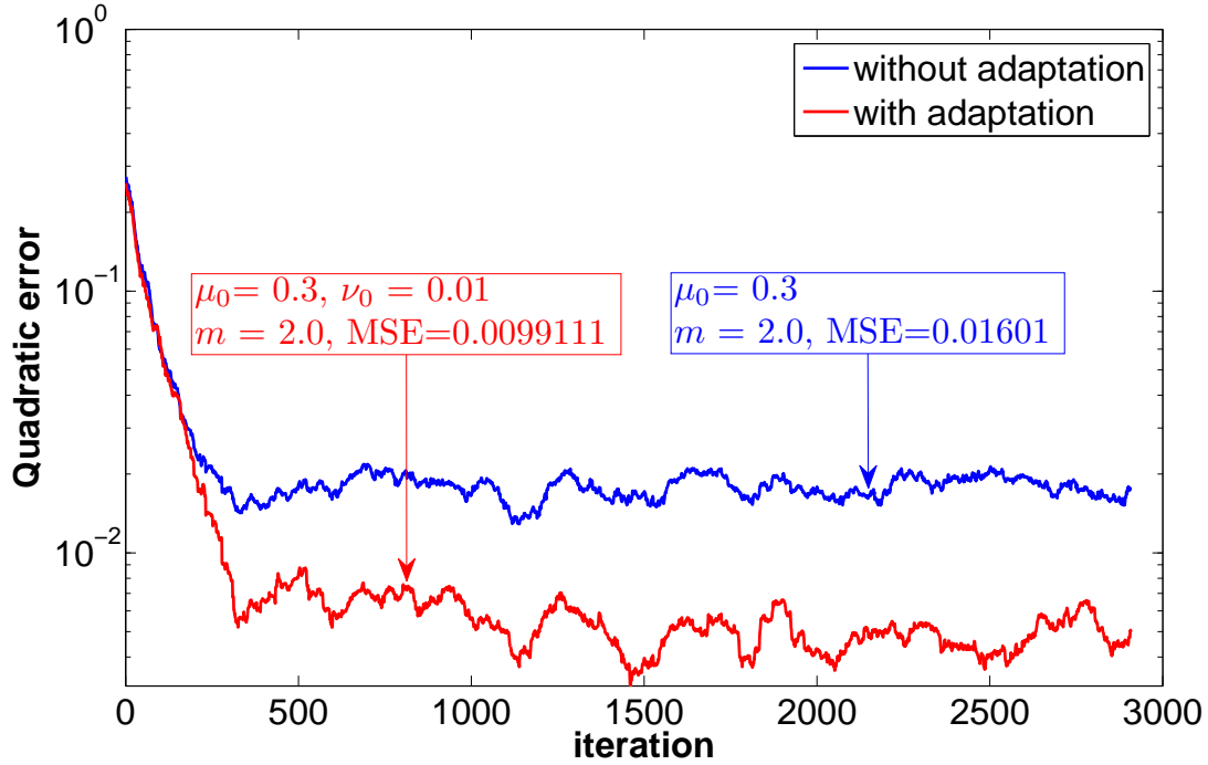
Figure 7. Logistic Map: Quadratic Error - KAPA with exponential kernel
