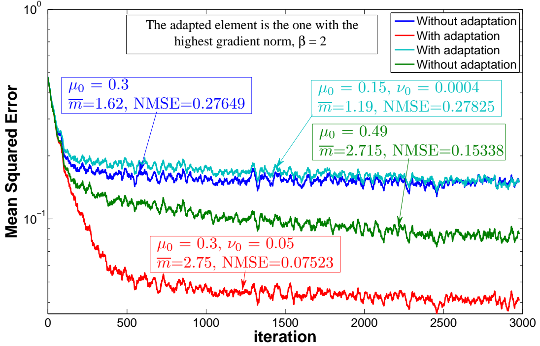
Figure 8. KAPA: Mean Squared Error with and without adaptation - Polynomial kernel ( \beta = 2 )
