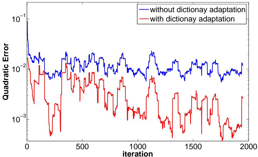
Figure 5. Quadratic error of Henon system modeling using KRLS with \mu_0 = 0.6 and \nu_0 = 0.05 .
