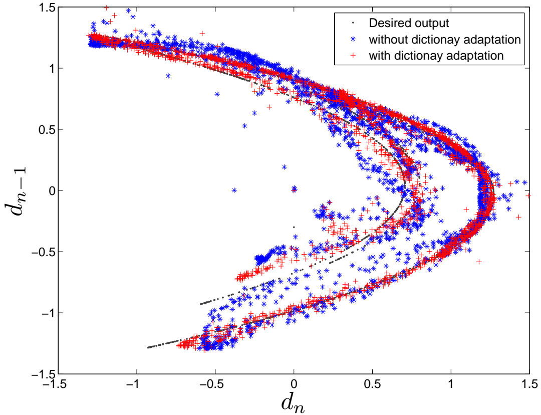
Figure 4. Henon system modeling using KRLS with \mu_0 = 0.6 and \nu_0 = 0.05 .
