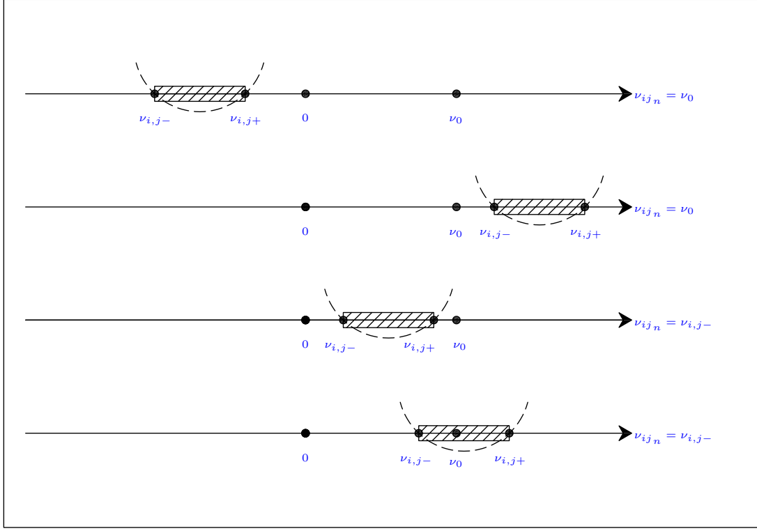
Figure 2. An illustration showing all the possibilities to select the gradient step size between any two dictionary elements \mathbf{u}_{w_i} and \mathbf{u}_{w_j} in the case of a radial basis kernel. \nu_0 > 0 is a reference step size.
