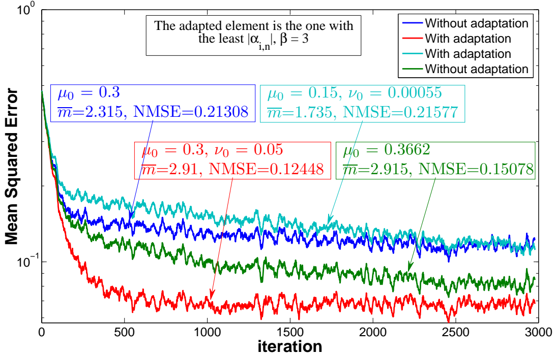
Figure 9. KAPA: Mean Squared Error with and without adaptation - Polynomial kernel ( \beta = 3 )
