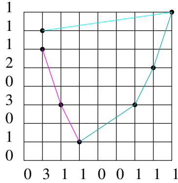
Figure 7: Encoding the grid lines.
