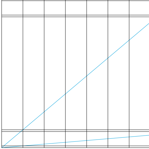
Figure 2: An 8 \times 8 grid without convex chains of size greater than 4 = \log 8 + 1 . X = \{0, 1, \dots, 7\} , Y = \{0, 1, 16, 17, 256, 257, 272, 273\} . Two lines through pairs of grid points are drawn in blue.
