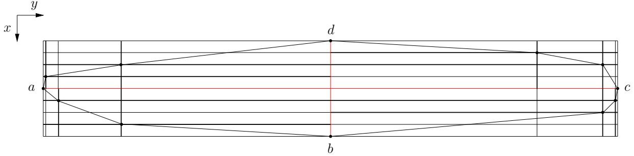
Figure 8: The n \times n grid defined in Section 4.2, with n = 9 = 2m + 3 for m = 3 , before doubling the median lines. The segments (parts of grid lines) incident to vertices are drawn in bold.
