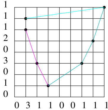
Figure 7: Encoding the grid lines.
