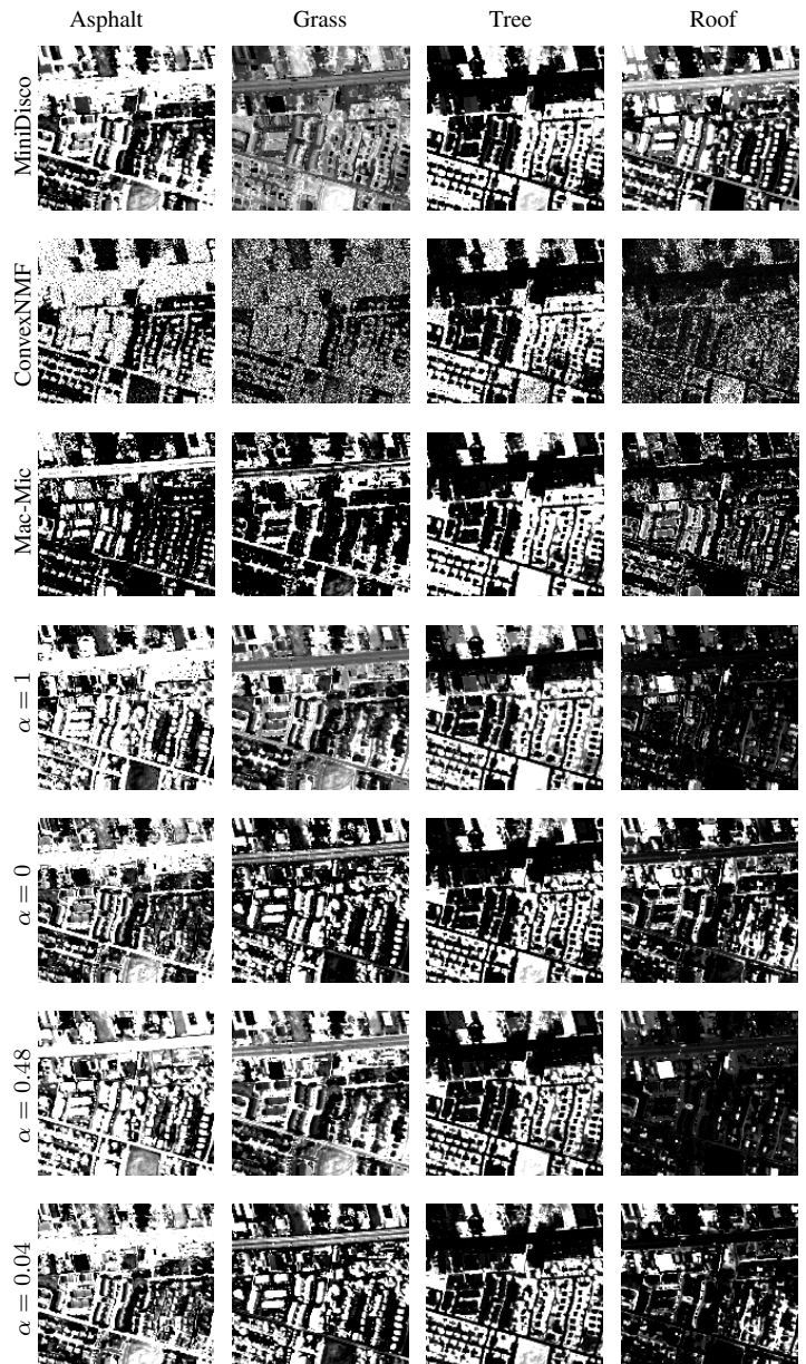
Fig. 9: Estimated abundance maps on the Urban image. Left to right: Abundance maps for Asphalt, Grass, Tree and Roof. Top to bottom: MiniDisco, ConvexNMF, Mac-Mic, and the proposed bi-objective NMF with \alpha = 1 (linear NMF), \alpha = 0 (nonlinear Gaussian NMF), and Pareto optimal solutions \alpha = 0.48 ( \ell_1/\ell_2 -norm), \alpha = 0.04 ( \ell_{-\infty} -norm).
