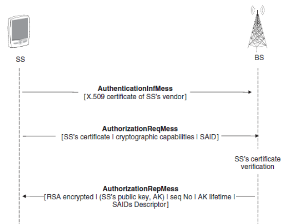
Fig 1 : PKM Authorization [14]
