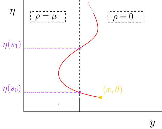
FIGURE 4. Sketch of a C-turn as the trajectory crosses the line twice. From Lemma 5.2, we see that this trajectory cannot be optimal.
