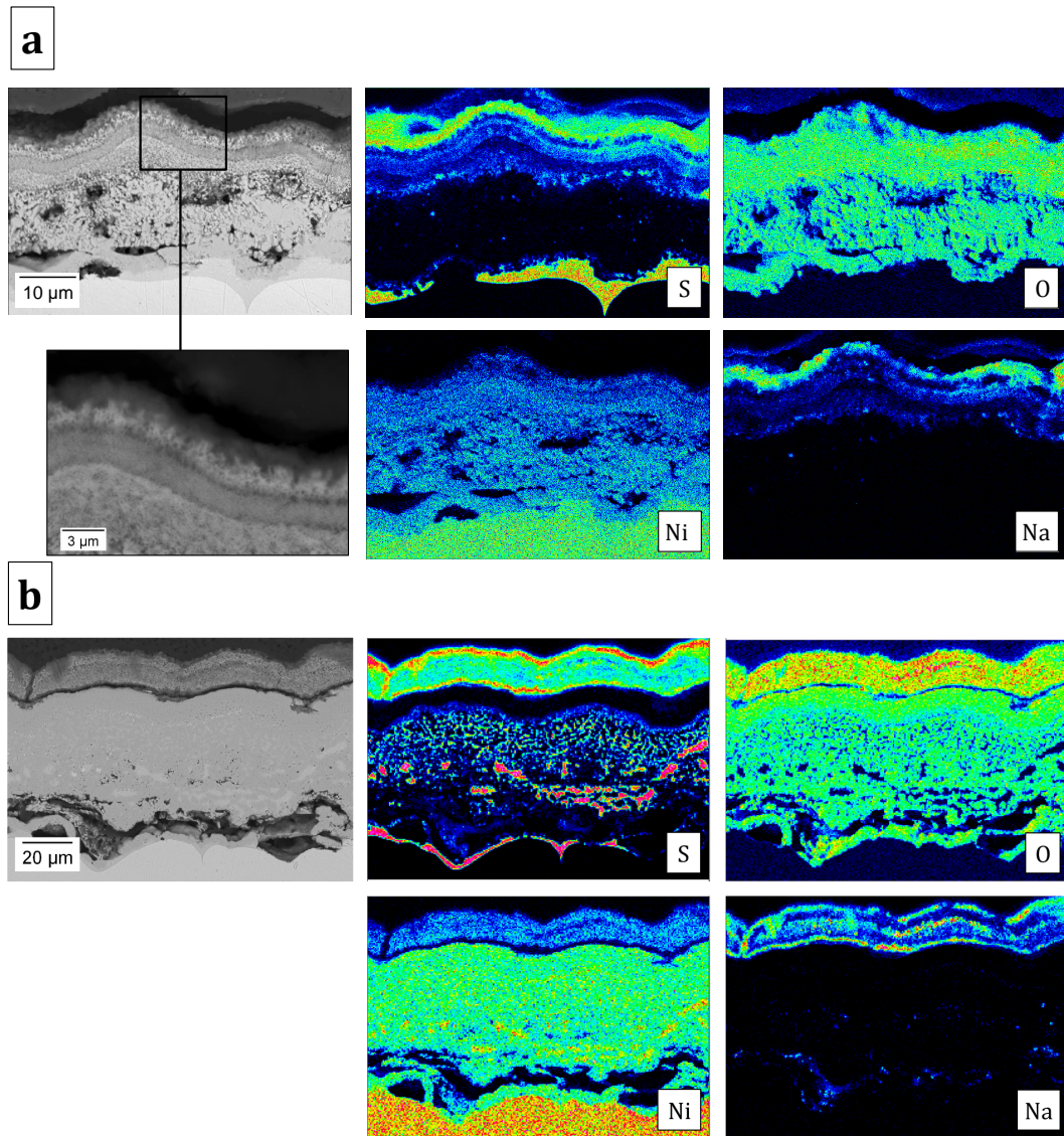
Figure 5: Back-scattered electron images and WDS maps of corrosion product formed after 6.5 h reaction of nickel with Na 2 SO 4 in O 2 -0.1SO 2 at 700 °C. The two regions come from the same specimen but reflect different stages of the reaction process: (a) in an earlier stage, the porous NiO scale is infiltrated with a Na 2 SO 4 -NiSO 4 solution in its top half (inset shows fine porosity in outer part); (b) in a later stage, the scale mostly contains a NiO + Ni 3 S 2 mixture.
