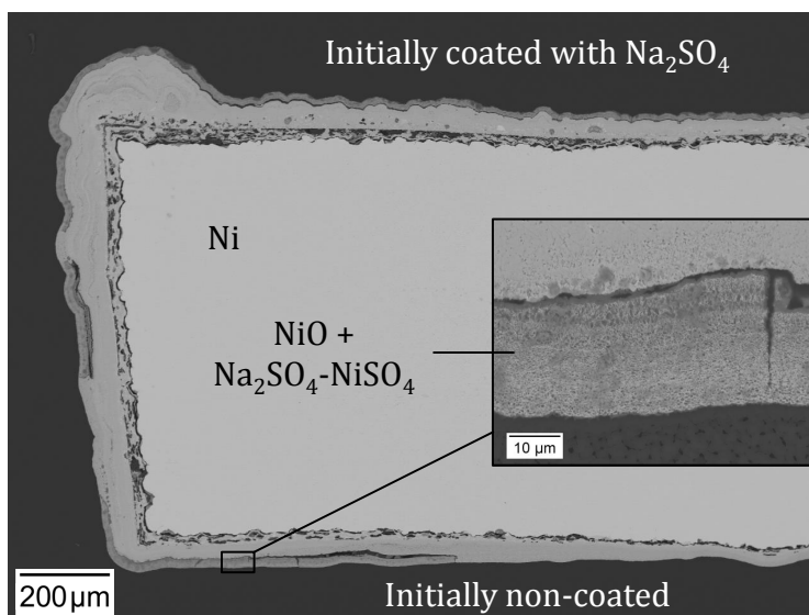
Figure 2: Cross-section of nickel specimen after 6.5 h reaction with \text{Na}_2\text{SO}_4 in \text{O}_2\text{-}0.1\text{SO}_2 at 700\text{ }^\circ\text{C} . The oxide scale on the bottom face (i.e., the side which was not coated with \text{Na}_2\text{SO}_4 prior to exposure) is infiltrated with \text{Na}_2\text{SO}_4\text{-NiSO}_4 , which indicates that the sulfate mixture was liquid at temperature.
