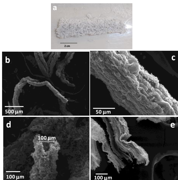
Fig.6 Image (a) and SEM pictures of replica TiO 2 Luffa sponges (TiO 2 -L) (b-e).
