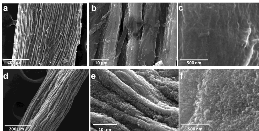
Fig.3 SEM pictures of treated Luffa fibers before (a-c) and after TiO 2 deposition (d-f).
