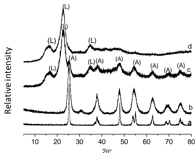
Fig.2 X-ray diffraction patterns for TiO 2 samples (a) standard, (b) TiO 2 powder recovered after the synthesis, (c) TiO 2 deposited on Luffa fibers (d) Luffa fibers.
