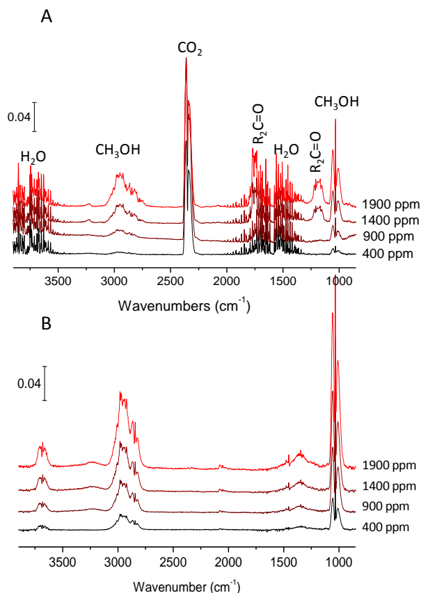
Fig.10 A) Evolution of the IR spectra of the gas phase during the photooxidation of methanol at different concentrations on TiO 2 /Luffa composite. (Flow= 25cm 3 /min, I 0 =25%). B) IR spectra of the gas phase before UV-irradiation of TiO 2 /Luffa composite pellet, at different methanol concentrations.
