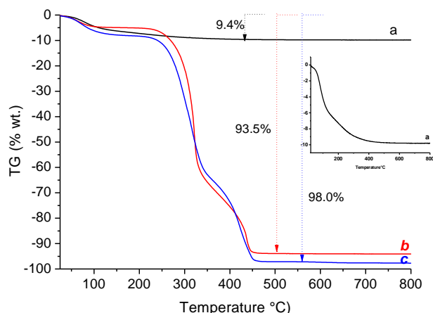
Fig.4 Thermogravimetric curves of: (a) as-synthesized \text{TiO}_2 , (b) \text{TiO}_2 /Luffa and (c) Luffa. Insert: full scale of the thermogravimetric curves as-synthesized \text{TiO}_2 .
