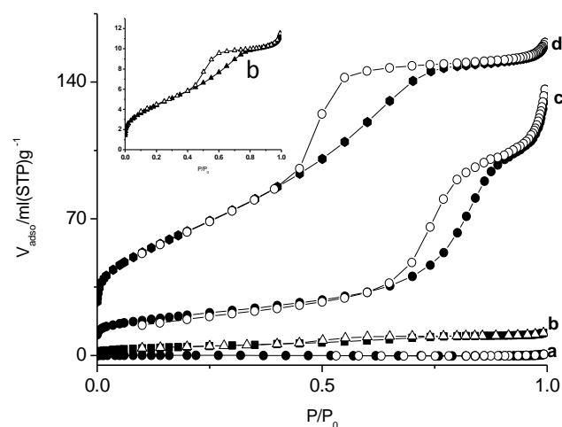
Fig.7 Nitrogen sorption isotherms adsorption (close symbols) and desorption (open symbols) at 77 K for : (a) Luffa fibers, (b) TiO 2 /luffa composites, (c) TiO 2 -L and (d) TiO 2 powder (the TiO 2 powder recovered after the synthesis).
