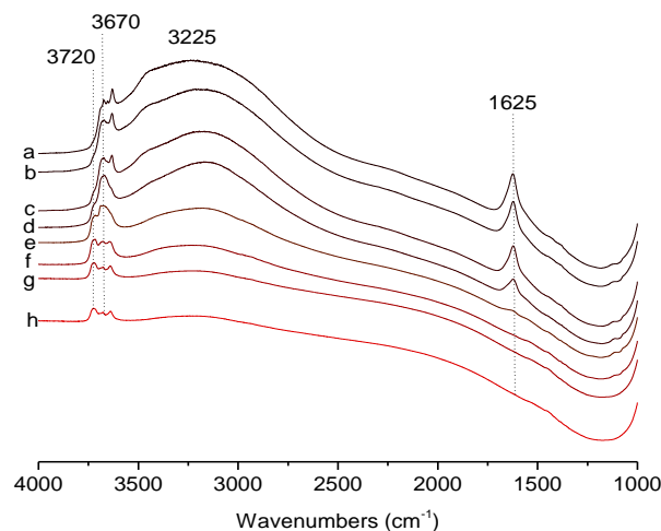
Fig.5 IR spectra of as-synthesized \text{TiO}_2 at RT under air (a) and under vacuum (b-h) at RT 50°C (b), 75°C (d), 125°C (e), 200°C (f), 300°C (g) and 350°C (h).
