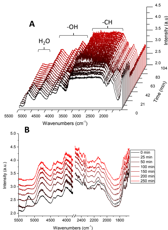
Fig.9 Evolution of the IR spectra of TiO 2 /Luffa surface during methanol photooxidation under operando conditions. (Flow= 25 cm 3 /min, MeOH/O 2 /Ar 400ppm/20%/79.99%, I 0 =25% ~2.5 mW/cm 2 at 366nm).
