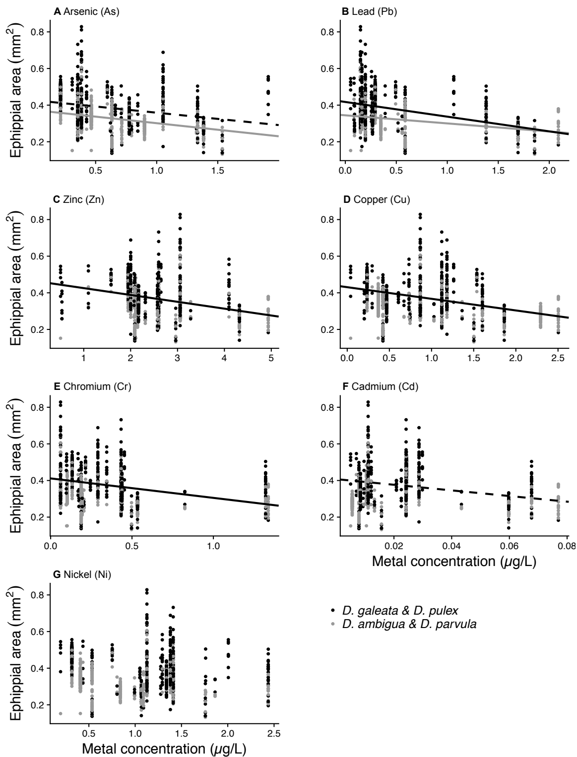
Fig. 2 Ephippial area (mm 2 ) according to metals concentrations (µg/L) in water ponds.
