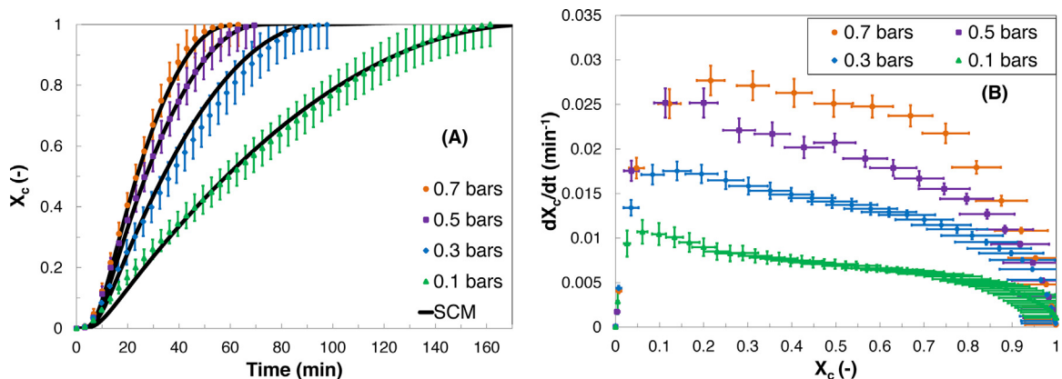
Fig. 12 – Effect of steam partial pressure on the (A) conversion rate versus time, (B) instantaneous gasification rate versus conversion rate, (experiments G.5).
