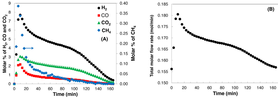
Fig. 3 – (A) Molar percentages of the non-condensable gases versus time, (B) total molar flow rates versus time, (experiment G.4c, \dot{n}_{N_2} = 0.155 \text{ mol min}^{-1} ).
