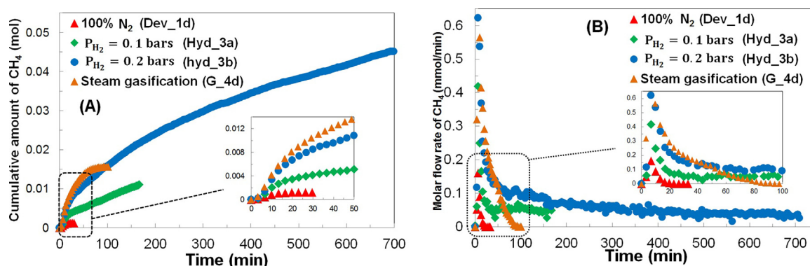
Fig. 9 – Effect of hydrogen partial pressure on (A) the cumulative amount of CH 4 (B) the molar flow rate of CH 4 (experiments Dev_1d, Hyd_3 and G_4d).
