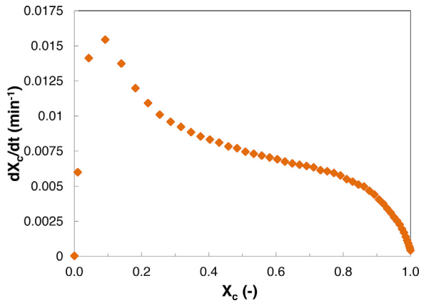
Fig. 4 – Instantaneous gasification rate versus carbon conversion rate, (experiment G.4c).
