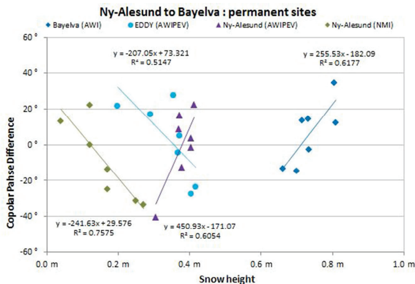
Figure 6: Copolar Phase Difference (CPD) and snow depth comparison: output results for 4 meteorological stations under different types of snow metamorphism during winter and spring 2017. Seven TerraSAR-X dates without melting conditions are taken in account.
