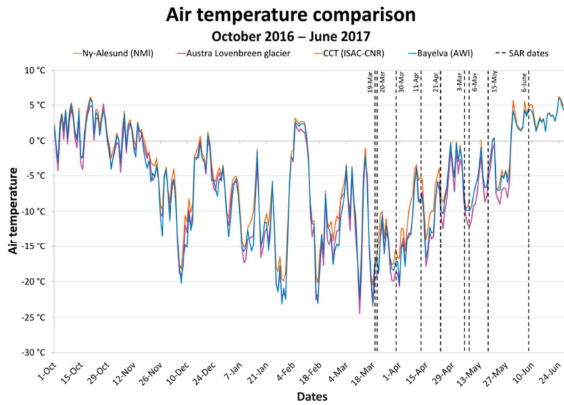
Figure 1: Air temperature temporal evolution, winter season 2016-2017, for four meteorological sites in Ny Ålesund area. TerraSAR-X acquisition dates are indicated in dashed lines (Source: AWI, ISAC-CNR, NMI, UFC).
