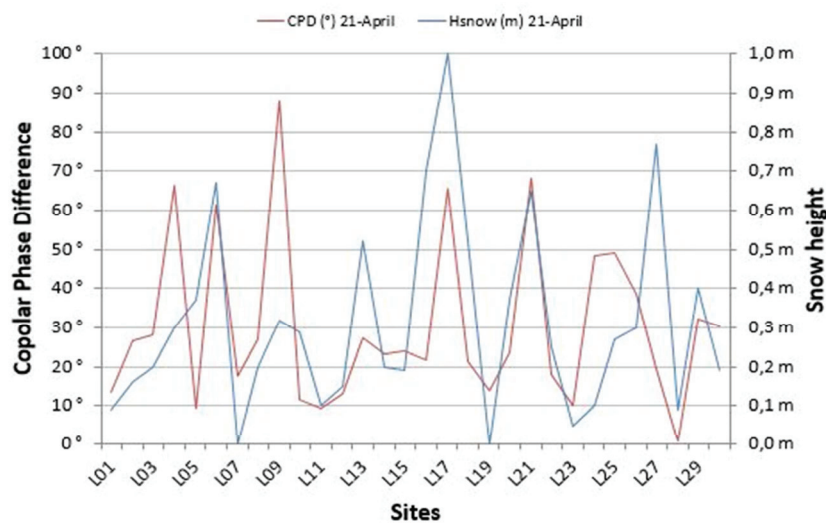
Figure 5: Copolar Phase Difference (CPD) and snow depth comparison: example of a snow line transect (manual collection) from Ny-Ålesund village to Bayelva meteorological station, 21/04/2017 (Source: AWIPEV).
