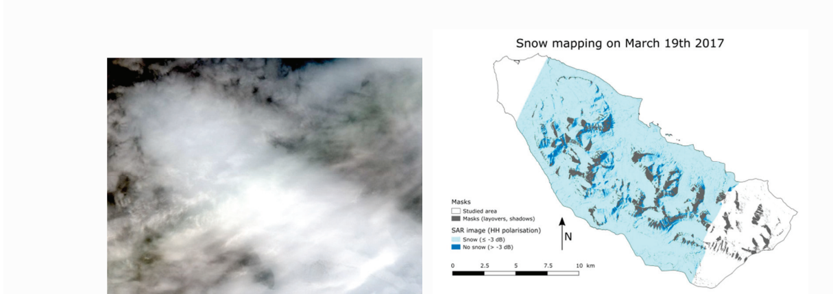
Figure 4: Cloud cover conditions: (a) on the left Sentinel-2 image of 19/03/2017, unusual for snow mapping; and (b) on the right TerraSAR-X acquisition, Nagler processing, successful at same day.
