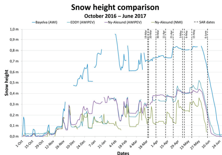
Figure 2: Snow depth temporal evolution, winter season 2016-2017, for permanent meteorological sites in Ny Ålesund area. TerraSAR-X acquisition dates are indicated in dashed lines (Source: AWI, AWIPEV, NMI).
