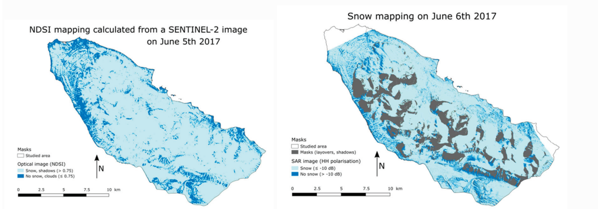
Figure 3: Cloud-free conditions: snow mapping comparison between (a) on the left Sentinel-2 image, NDSI processing, at 05/06/2017; and (b) on the right TerraSAR-X, Nagler processing, at 06/06/2017.
