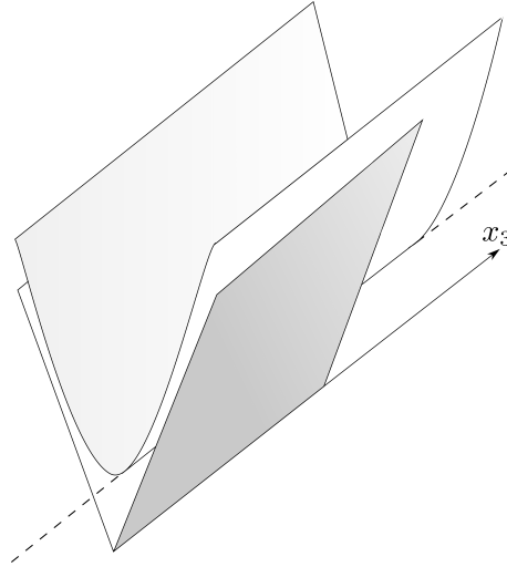
Figure 14.1: The "book" approximation
