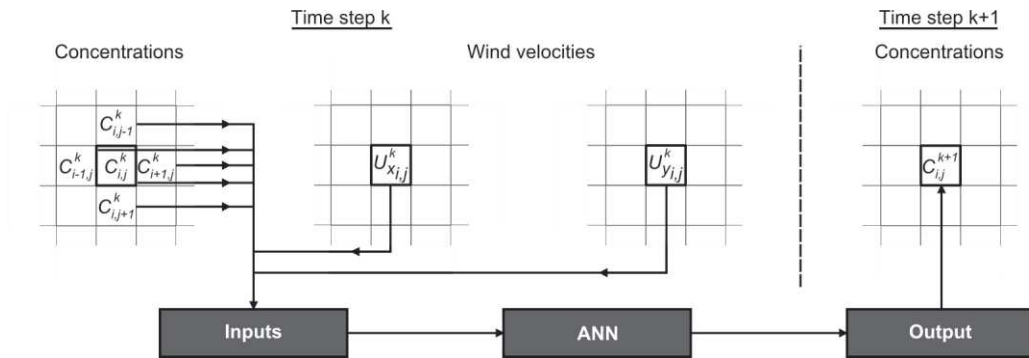
Figure 4: CA transition rule algorithm
