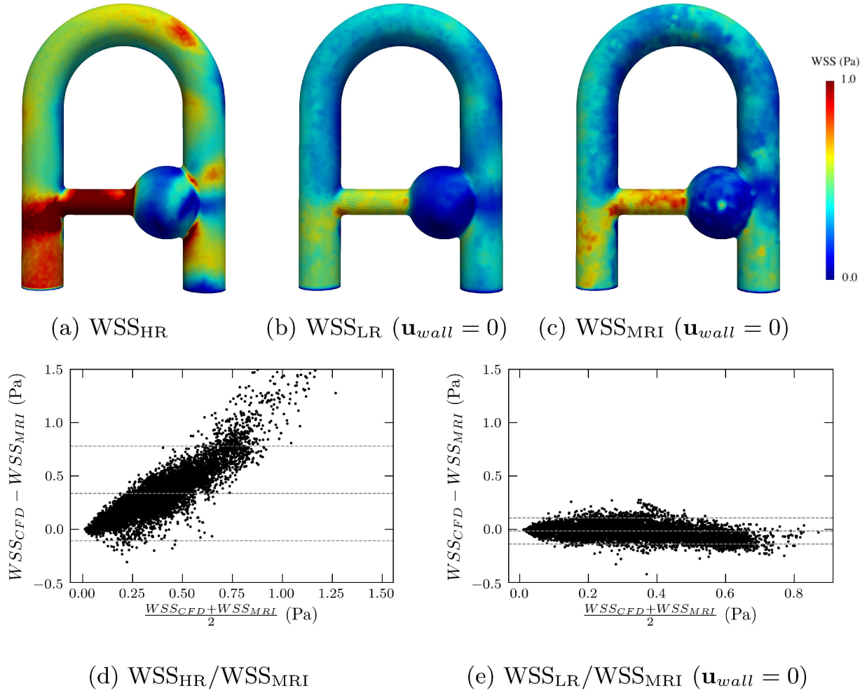
FIGURE 9 Wall Shear Stress maps on boundary walls at peak systole. (a) WSS calculated from the HR CFD velocity field, (b) from the LR CFD velocity field (with zero velocity imposed on boundary walls) and (c) from the PC-MRI velocity field (with zero velocity imposed on boundary walls). Bland-Altman plots of the comparison between (d) WSS_{HR} and WSS_{MRI} (corresponding to r_{WSS}^2 = 0.48 in Table 4 ) and (e) WSS_{LR} and WSS_{MRI} corresponding to r_{WSS}^2(\mathbf{u}_{wall} = 0) = 0.84 in Table 4 .
