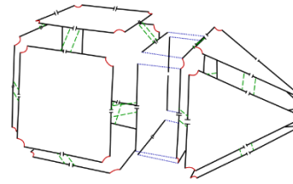
Figure 2: Two darts sewed by \alpha_0 link form an edge (black lines). Several edges sewed by \alpha_1 links (red curves lines) form a face. Several faces sewed by \alpha_2 links (green large dotted lines) form a volume. Several volumes sewed by \alpha_3 links (blue thin dotted lines) form one connected component.
