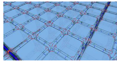
Figure 5: The 3D volume topological model is inspired from the building process employed in the physics' model: 70 \times 70 \times 10 topological cubic volumes are sewed to each other's.
