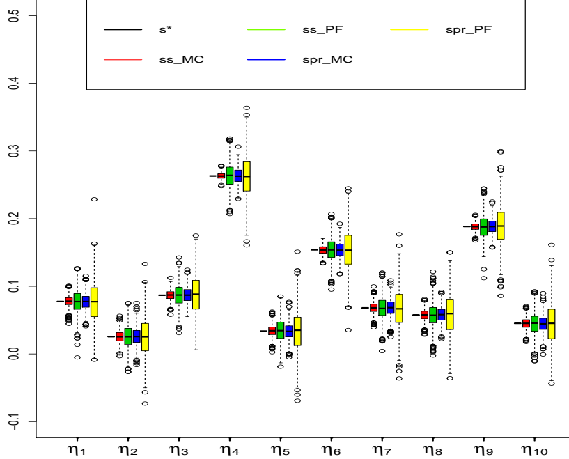
Figure 1: Estimation of the Shapley effects in the linear Gaussian framework. In black ( s^* ) we show the theoretical values, in red ( ss\_MC ) the estimates from the subset W -aggregation procedure with the double Monte-Carlo estimator, in green ( ss\_PF ) the estimates from the subset W -aggregation procedure with the Pick-and-Freeze estimator, in blue ( spr\_MC ) the estimates from the random-permutation W -aggregation procedure with the double Monte-Carlo estimator and in yellow ( spr\_PF ) the estimates from the random-permutation W -aggregation procedure with the Pick-and-Freeze estimator.
