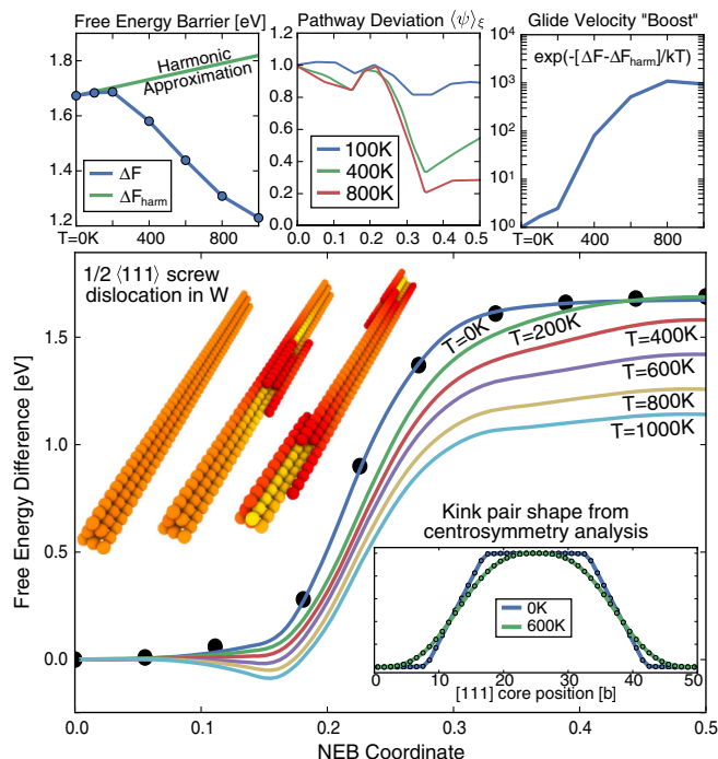
FIG. 2. Free energy for double kink nucleation for a \langle 111 \rangle screw in W . Inset: Kink profile determined through centrosymmetry analysis on the time averaged atomic positions [51]. Top left: Kink formation free energy. Top center: Pathway deviation \langle \psi \rangle_{\xi} . Top right: Effective “boost” in the expected glide velocity due to anharmonic corrections.
