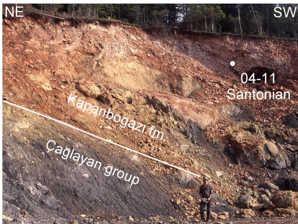
Fig. 12: Unconformity of the Kapanbogazly red pelagic limestone (Santonian, samples 04-11, 15, 16) on the Çağlayan sandstone (Hauterivian-Barremian, samples 04-12, 13, 19) near Ağlıköy (Fig. 4).
