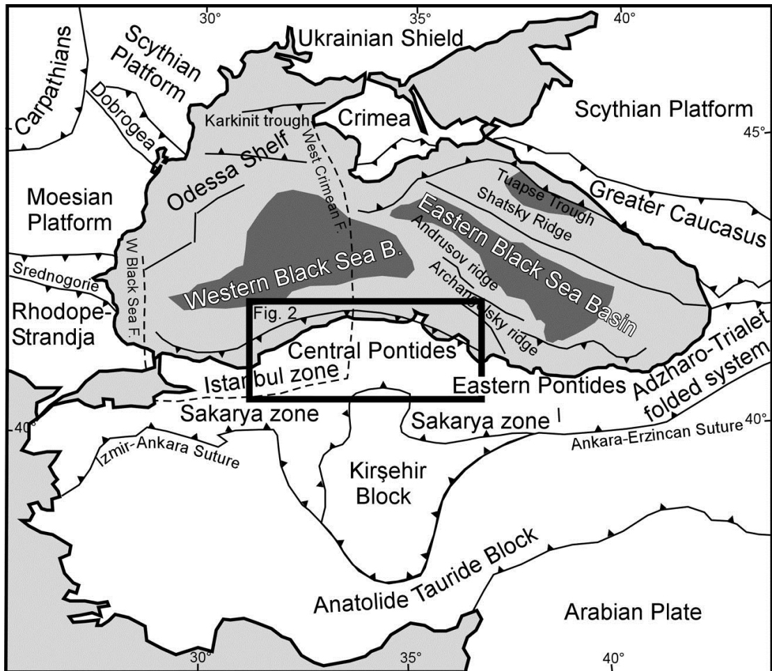
Fig. 1: Location of the arc of Central Pontides between the Western Black Sea Basin and the Kirsehir Block (modified after Robinson et al., 1996; Robinson, 1997; Okay and Tüysüz, 1999).
