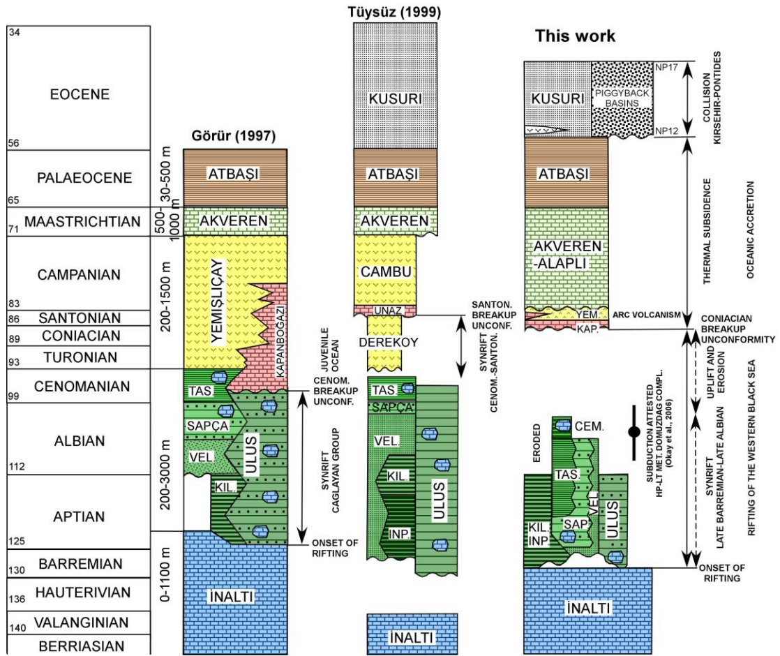
Fig. 3: Comparison of dating of the stratigraphic formations of the Central Pontides (Black Sea coast, Zonguldak Basin and Ulus Basin). CEM: Cemaller Formation; İNP, İnpiri Formation; KAP: Kapanboğazı Formation; KIL: Kilimli Formation; SAP: Sapça; TAS: Tasmaca Formation; YEM: Yemişliçay Formation; VEL: Velibey Formation.
