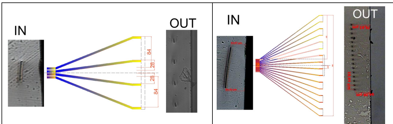
Fig. 5: Left, 1x4 lantern, where separation between channels is 60 \mu m. Right, 1x16 lantern, with 20 \mu m separation. A second set with 1x4 and 20 \mu m separation and 1x16 with 60 \mu m separation was also fabricated (see fig. 6).
