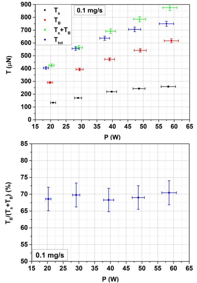
Figure 5. Top: direct measurement of the thrust applied on the source T_S , on the magnet T_B , T_S + T_B , and total measured thrust T_{tot} versus injected power. Bottom: ratio of magnetic thrust T_B to the sum T_S + T_B versus the injected power. Q_m = 0.1 \text{ mg/s}
