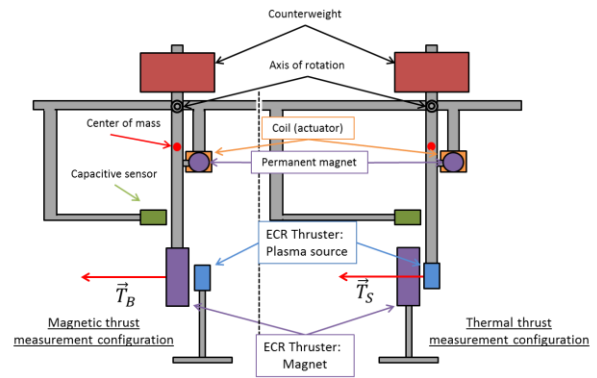
Figure 3. Schematic of the thrust balance adapted for the separate measurement of the thrust components
