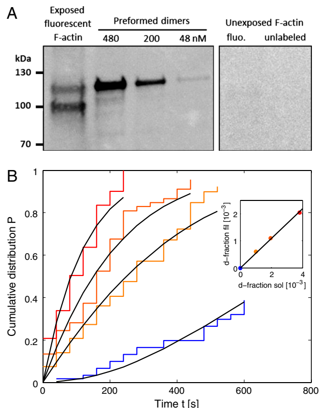
Fig. 4. Illumination of fluorescently labeled F-actin creates actin dimers as revealed by comparison with preformed, covalently cross-linked dimers. (A, Left) Western blots obtained with an actin antibody. The apparent molecular masses of the photo-induced dimers (left column) are compared with the corresponding masses of the preformed dimers (three columns on the right corresponding to three different bulk concentrations of preformed actin dimers). The apparent mass of the actin dimers exceeds their true mass of 86 kDa because the cross-links lead to a branched polypeptide chain. (A, Right) No dimers could be detected in labeled or unlabeled F-actin solutions that were not exposed to light. (B) Cumulative distributions for the occurrence of pauses during the depolymerization of filaments grown from G-actin with labeling fraction X_{\text{fl}} = 0.1 in the presence of 0 (blue data), 2, 4, and 8 nM (three sets of reddish data) preformed actin dimers. The black lines represent calculated distributions as described in SI Text on Theoretical Analysis . The Inset shows the linear relationship between the mole fractions of the preformed dimers (d-fractions) in the filaments and in solution.
