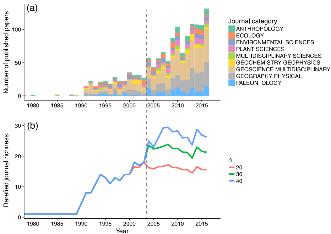
Figure 1. Meta-analysis of published scientific articles ( n = 960 ) containing the terms “paleo **” and “charcoal” from the Thompson ISI Web database between 1980 and 2016. (a) Number of published articles by year and corresponding ISI web journal categories. (b) Diversity of the journals publishing articles with the keywords “paleo **” and “charcoal” assessed using rarefied journal richness (Birks & Line, 1992) [13]. For each year under analysis, the rarefied journal richness was computed with constant annual publication sums of 20, 30, and 40 articles; i.e., journal diversity was standardized in order to take into account publication volume growth during the studied period.
