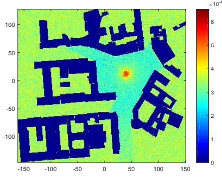
Fig. 7. Heat map of bad user configurations with simulation parameters \epsilon = 0.3 and \lambda = 2^{-12} (or \lambda \approx 2.44 \times 10^{-4} ), and \tau = -50 (or \tau_\lambda = -13.88 ) dB. The average user density is estimated for the atypical event of a large fraction of disconnected users. The regions of higher values show where users tend to be located during bad configurations. Naturally, these include regions far or hidden from the target base station. But there is also a region around the base station, due to the so-called near-far effect, where too many users have decreased the SIR values of the remaining network users.
