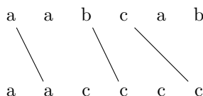
■ Figure 4 An alignment between T = aabcbab and S = aacccc of cost 7.
