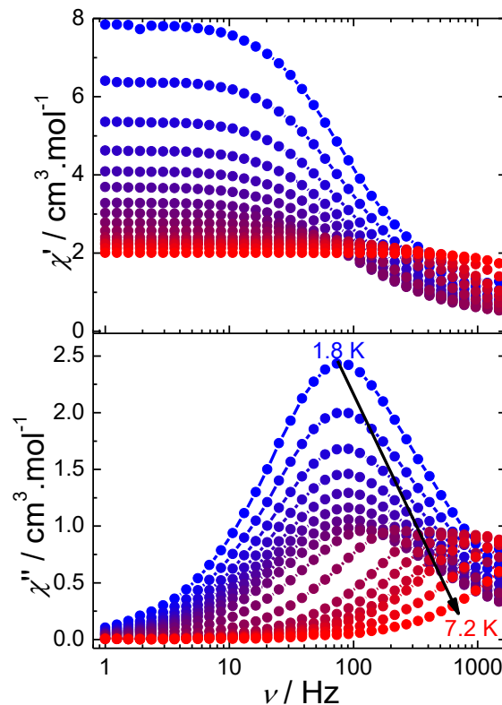
Fig. 2. Frequency dependence of the in-phase ( \chi' ) and out-of phase ( \chi'' ) susceptibilities for 1 under a zero dc-field.
