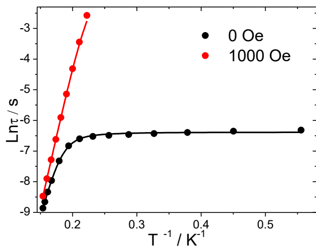
Fig. 3. Temperature dependence of the relaxation time for 1 using the ac susceptibility data at 0 Oe and 1000 Oe. The solid line represents the fit with Eq. 1 (0 Oe) and Eq. 3 (1000 Oe).
