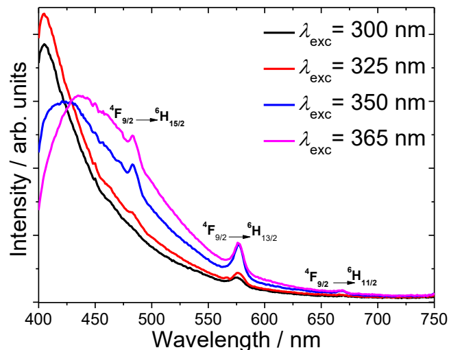
Fig. 4. Room temperature solid-state emission spectra of 1 acquired at different excitation wavelengths. The intra 4f^3 \text{ Dy}^{3+} transitions are reported.
