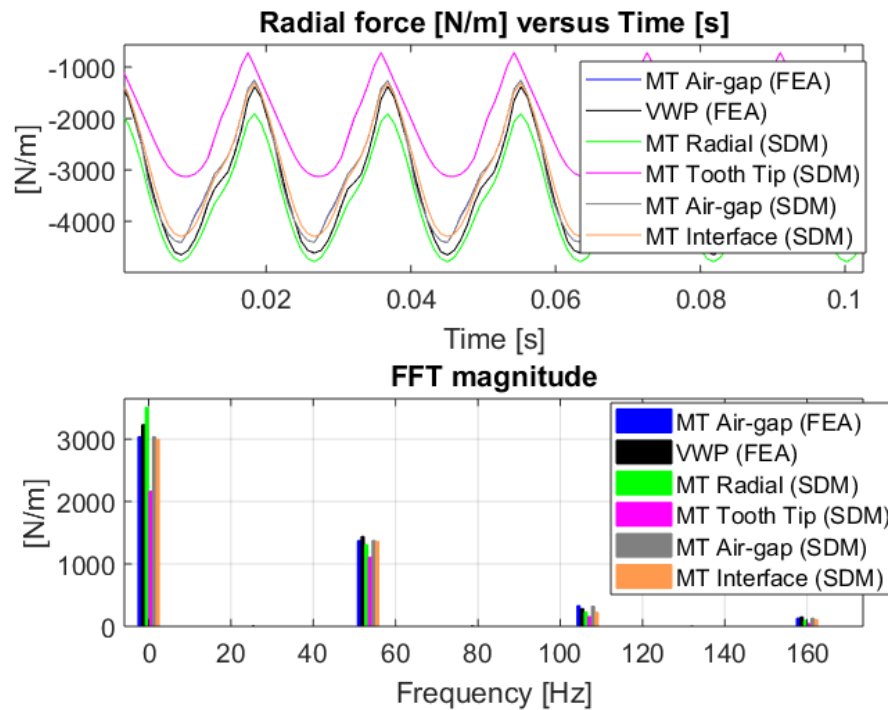
Fig. 12. Radial lumped force during one revolution and its FFT according to different methods with a linear B-H curve
