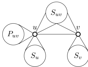
Figure 4: The structure of a D2C graph with the dominating edge uv (the only edges that are depicted are those incident with u or v ). Lemma 7 allows us to represent all vertices in P_{uv} as adjacent to u .
