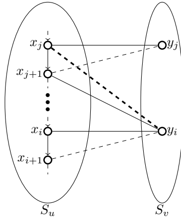
Figure 9: Illustration of the proof of Lemma 14: x_j is the first predecessor of x_i in the cycle such that x_j y_i \notin E . The non-edge \overline{x_j y_i} is then f -free.
