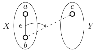
Figure 5: The construction of the function f . The edge e = ab is critical for the pair \{b, c\} , thus f(e) = \overline{bc} .
