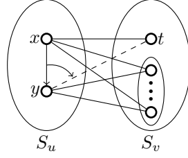
Figure 8: Illustration of Lemma 13: if x and y are two vertices in S_u (resp. S_v ) such that \vec{xy} is an arc of the f -orientation and neither x nor y is incident with an f -free non-edge, then the neighbourhood of x in S_v (resp. S_u ) is exactly the neighbourhood of y in S_v (resp. S_u ) plus one vertex.
