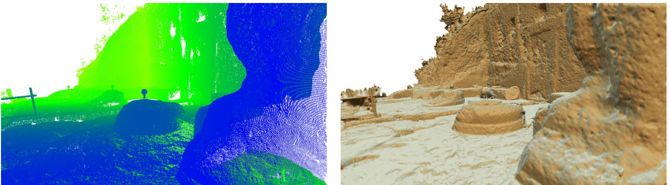
Figure 1: 73.6 million points laser scanned Scalina Etruscan tomb rendered with our algorithm at 120 fps. The surface ( right ) is reconstructed only from a depth buffer ( left ) by efficient pyramidal operators in real-time on the GPU.
