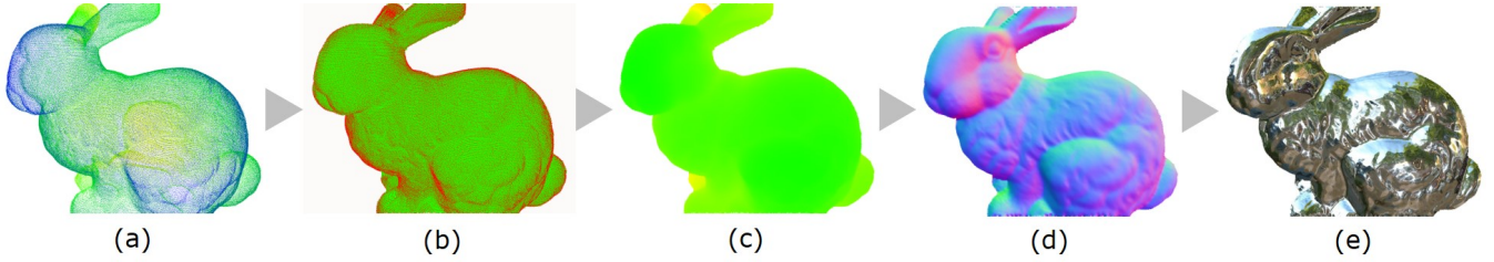
Figure 2: Overview of our method pipeline. (a) Geometry rendering with one pixel per point. (b) Hidden Point Removal (HPR), in red: foreground visible points, in green: hidden points. (c) Depth and attributes reconstruction [Kra09]. (d) Normals estimation. (e) Shading.
