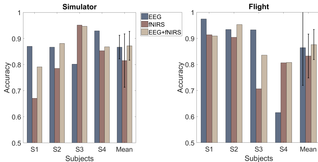
Fig. 2. Classification accuracy for all subjects and mean classification accuracy (vertical black bars represent standard deviation). Left: in the simulator condition. Right: in the real flight condition.
