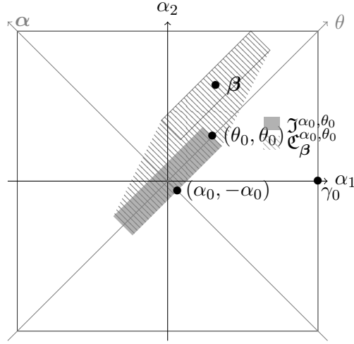
Figure 2: Schematic representation of the domains \mathcal{J}^{\alpha_0, \theta_0} \cap \mathbb{R}^\ell and \mathcal{C}_\beta^{\alpha_0, \theta_0} \cap \mathbb{R}^\ell for \ell = 2 compared to the constant \gamma_0 in the spin-fermion model.
