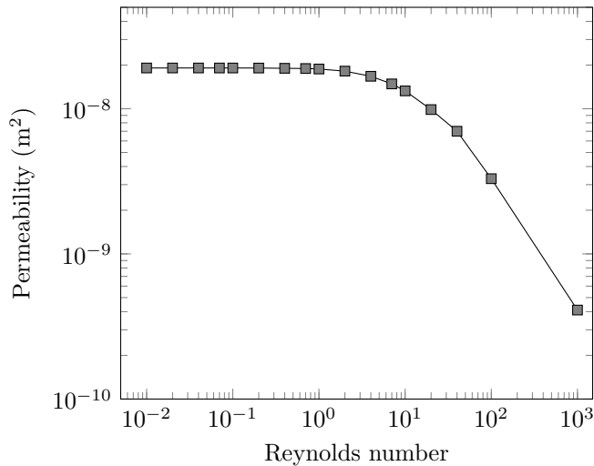
Figure 13: Computed permeability evolution with increasing Reynolds number
