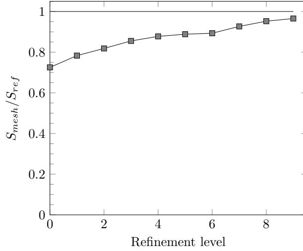
Figure 8: Mesh surface convergence with refinement level
