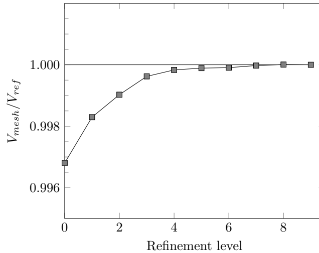
Figure 7: Mesh volume convergence with refinement level
