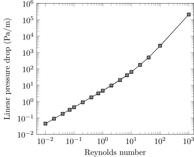
Figure 12: Pressure gradient evolution with increasing Reynolds number
