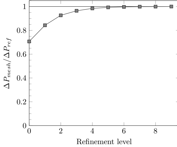
Figure 9: Pressure drop convergence with refinement level
