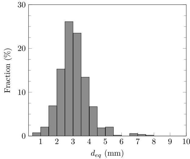
Figure 3: Equivalent diameters distribution. Total chip count: 536
