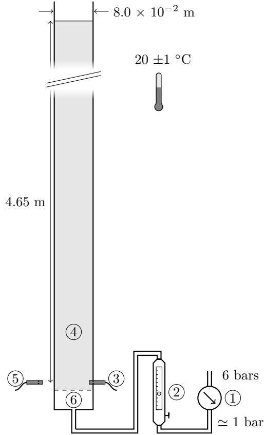
Figure 4: Experimental apparatus schematic. 1: pressure reducer, 2: flow controller, 3: bed pressure sensor, 4: wood chip bed, 5: room pressure sensor, 6: perforated grid ( 1 \cdot 10^{-3} m diameter holes)
