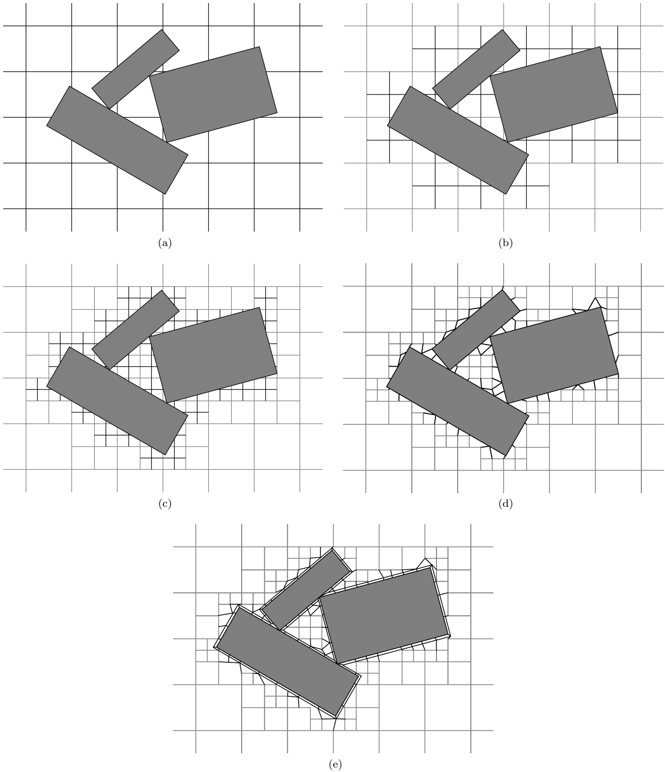
Figure 6: Meshing technique. (a) Background mesh and wood chips. (b) First refinement of the background mesh based of the intersection with the wood chips' surfaces. (c) Second refinement of the background mesh based of the intersection with the wood chips' surfaces. (d) Snapping of the refined mesh to the wood chips' surfaces. (e) Boundary layer addition
