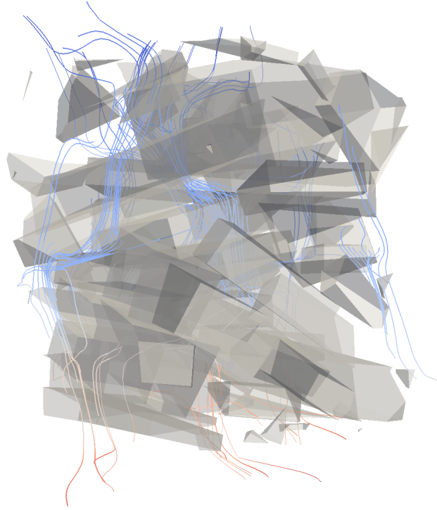
Figure 10: Upright flow visualization. Translucent gray: wood chips, colored lines: streamlines colored by pressure field values (seeds, two perpendicular horizontal lines crossing at the center of the sample)
