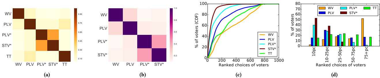
Figure 2: Heatmaps depicting the Jaccard Coefficients between different methods for selecting (a) trending topics in Twitter, and (b) most popular news in Adressa. (c) Average ranked choices and (d) Percentile choices for the trending topics selected by different methods throughout July, 2017.
