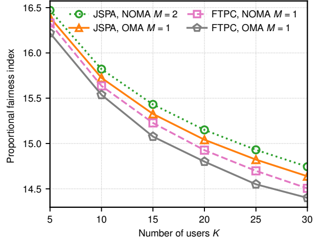
Fig. 6. Proportional fairness index of JSPA and FTPC
