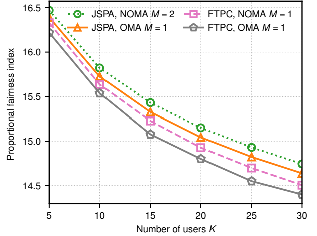
Fig. 6. Proportional fairness index of JSPA and FTFC
