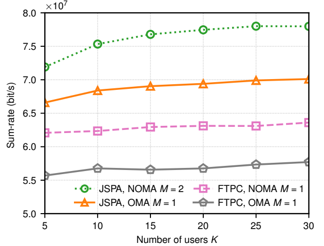
Fig. 7. Sum-rate of JSPA and FTFC in a proportional fair scheduler
