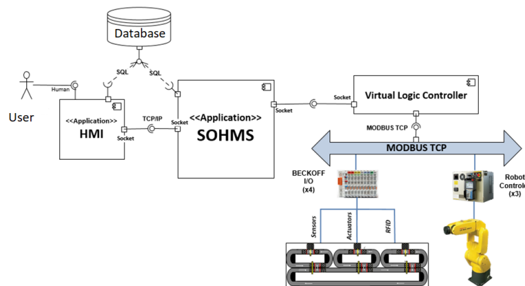
Fig. 1 Gamboa manufacturing software [?]
