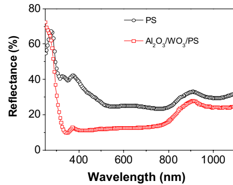
Fig. 6 Reflectance spectra of PS and Al 2 O 3 /WO 3 /PS samples
