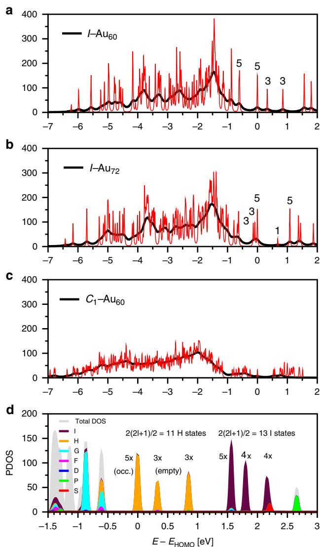
Fig. 3 Electronic-structure comparison of I\text{-Au}_{60} , I_h\text{-Au}_{60} , and C_1\text{-Au}_{60} clusters. a–c Electronic density of states (eDOS) of I\text{-Au}_{60} , I\text{-Au}_{72} , and C_1\text{-Au}_{60} clusters. Degeneracies are indicated by the numbers. To highlight both the general shape of the eDOS and the discreteness of some parts of it, we draw the eDOS convoluted with Lorentzians of different width, viz., with \Gamma = 0.1 (black) and 0.01 eV (red). The I\text{-Au}_{60} is clearly more strongly peaked and shows more strongly separated, degenerate levels around the HOMO-LUMO gap than the I\text{-Au}_{72} . The d band differs only little between these two structures. The eDOS of the two shell structures are very different from the much less peaked eDOS of the 3D C_1\text{-Au}_{60} where hardly any degeneracies are found. d Projected density of states of I\text{-Au}_{60} shell
