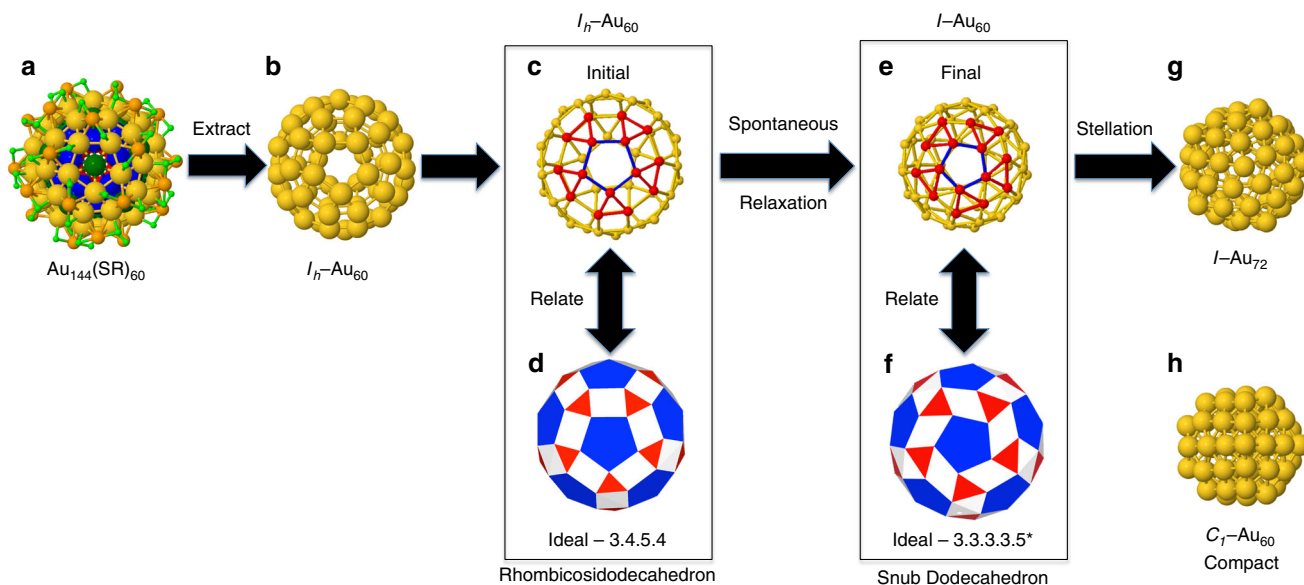
Fig. 1 Spontaneous formation of the I - Au_{60} shell. a Atomic structure of Au_{144}(SR)_{60} from reference 13 , b the I_h - Au_{60} constitutive shell derived from Au_{144}(SR)_{60} , c and e show the ball-and-stick atomic models of the Au_{60} shell before ( I_h - Au_{60} ) and after ( I - Au_{60} ) atomic relaxation. Some Au atoms located in two opposite pentagonal facets are displayed in different colors to show the structural transition. Note the significant contraction of the 60-atom Au shell. d Rhombicosidodecahedron and f Snub dodecahedron Archimedean polyhedra, g the I - Au_{72} nanoshell, and h compact C_1 - Au_{60} nanoparticle
