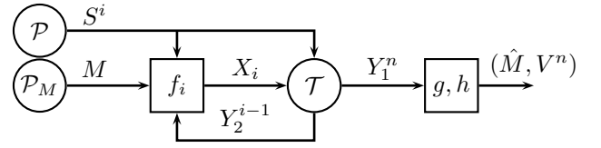
Fig. 4. The noisy feedback sequence Y_2^{i-1} is drawn i.i.d. according to \mathcal{T}_{Y_1Y_2|XS} . The encoding is f_i : \mathcal{M} \times \mathcal{S}^i \times \mathcal{Y}_2^{i-1} \rightarrow \mathcal{X} , \forall i \in \{1, \dots, n\} .
