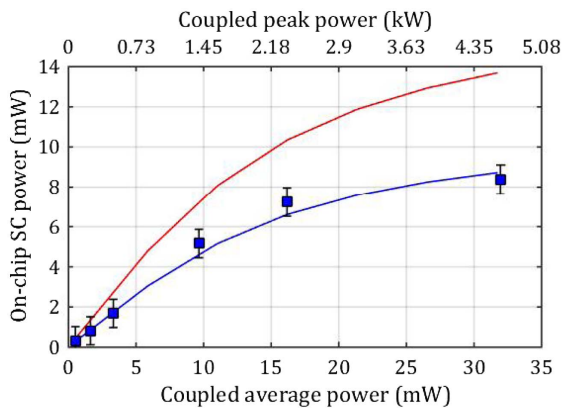
Fig. 5. On-chip SC power versus coupled average power measured for the 7 cm long waveguide (1) in TE at 4.0 μm (blue squares), simulated results for the 7 cm waveguide (blue line) and simulated results for a 2 cm long similar waveguide (red line).
