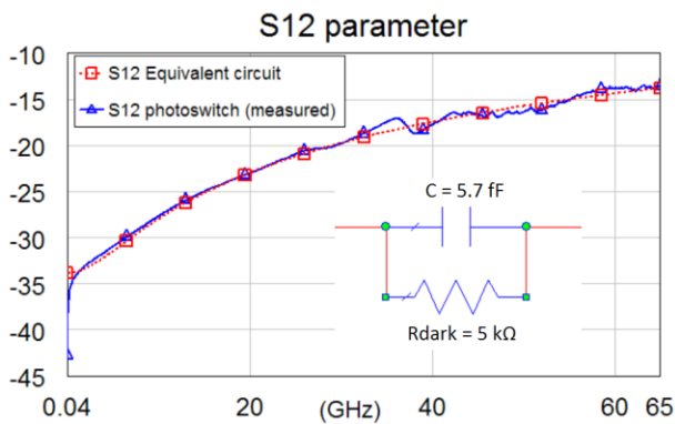
Fig. 2. S_{12} parameter of the PSW in the dark state. The inset shows the lumped elements equivalent circuit of the device.
