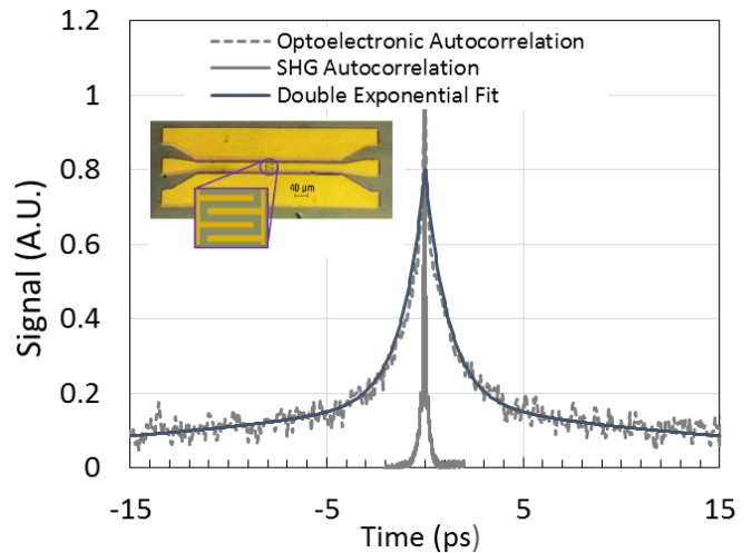
Fig. 1. Optoelectronic (dashed grey line) and optical (grey line) autocorrelation traces of a Nitrogen implanted InGaAs PSW (inset). A double exponential fitting curve with time constants of .2 and 20 ps is also shown (black line).
