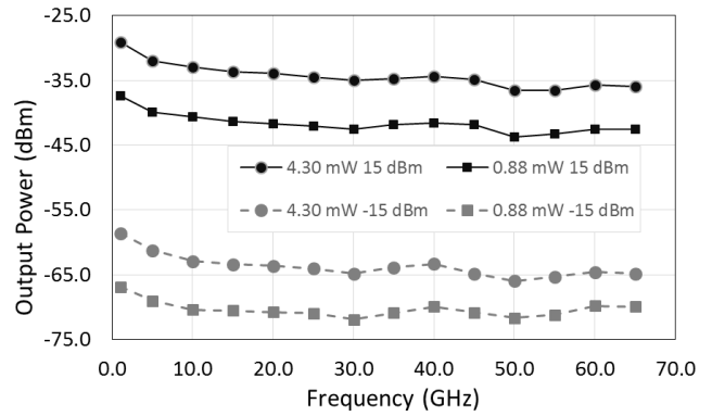
Fig. 3. Output power of the sampled signal for different experimental conditions: average optical power of 4.3 or 0.88 mW and RF power of - 15 dBm or + 15 dBm. The x axis represents the frequency of the RF input signal.
