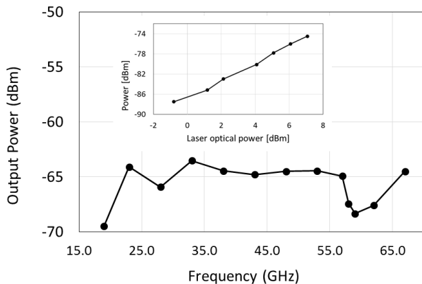
Fig. 4. Power of the IF signal for different input RF frequencies. The PSW is used as a heterodyne mixer in between a 14 dBm RF input signal and a 5 mW optical beam self-oscillating at 58.625 GHz. The inset shows the IF power dependence onto the optical power.
